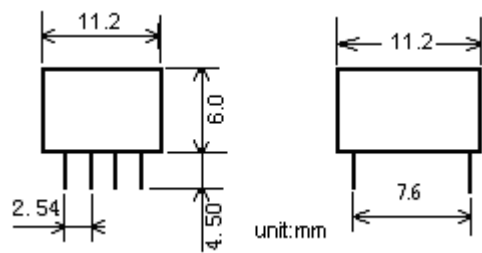
SD2403 ,DIP8 Package
